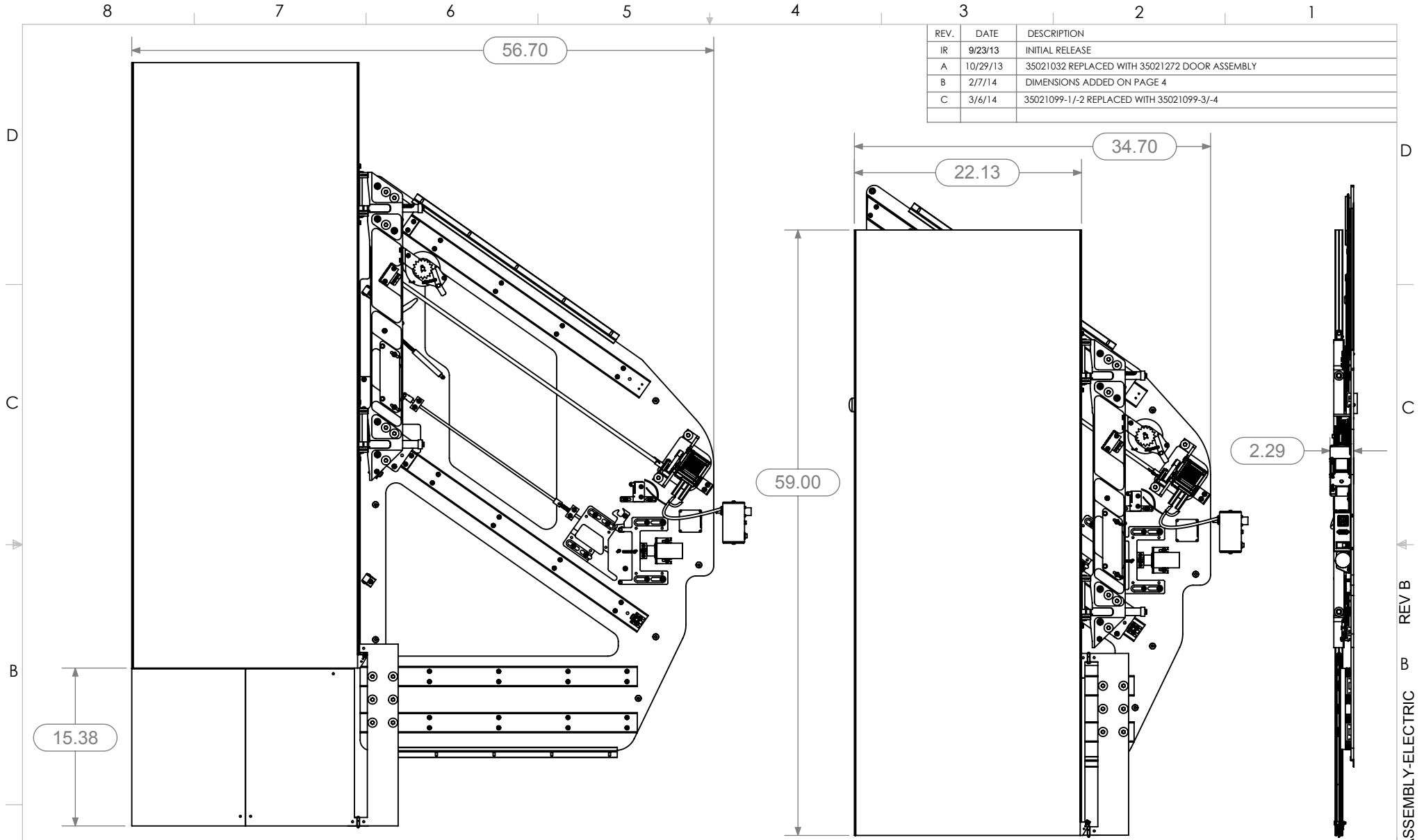
DETAIL-1 POCKET DOOR ASSEMBLY STOWED
